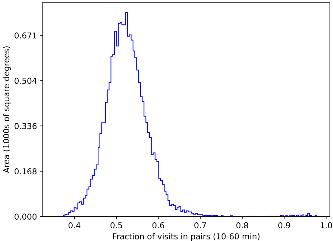
all_long_v3.4_10yrs gri WFD: Fraction of visits in pairs (10-60 min)
