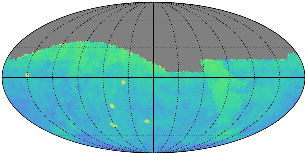
all_long_v3.4_10yrs gri All sky: Fraction of visits in pairs (10-60 min)
