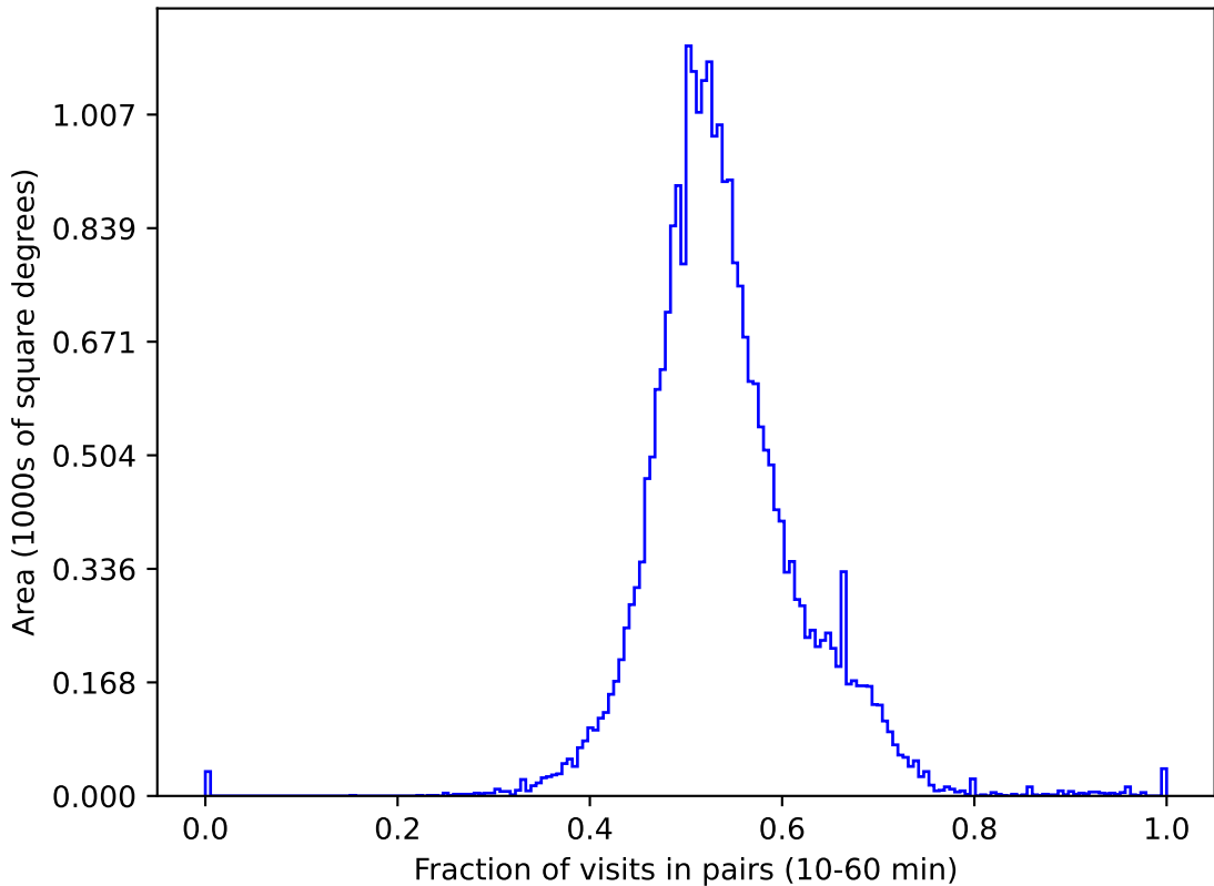
all_long_v3.4_10yrs gri All sky: Fraction of visits in pairs (10-60 min)
