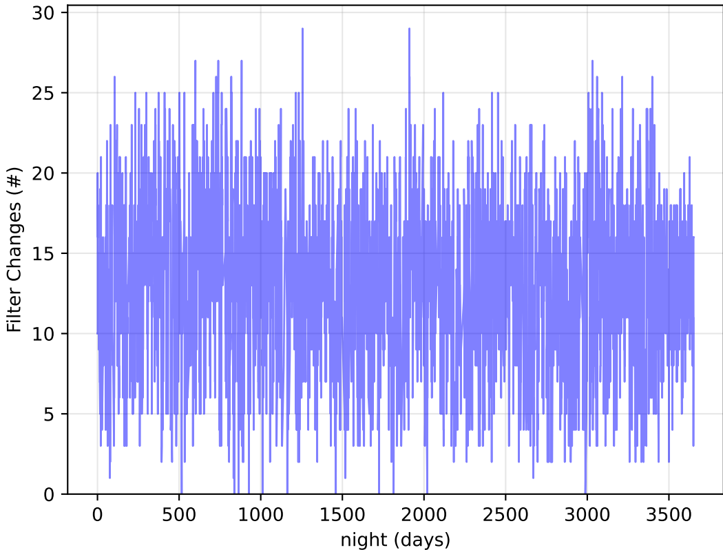
all_long_v3.4_10yrs Per Night: Filter Changes
