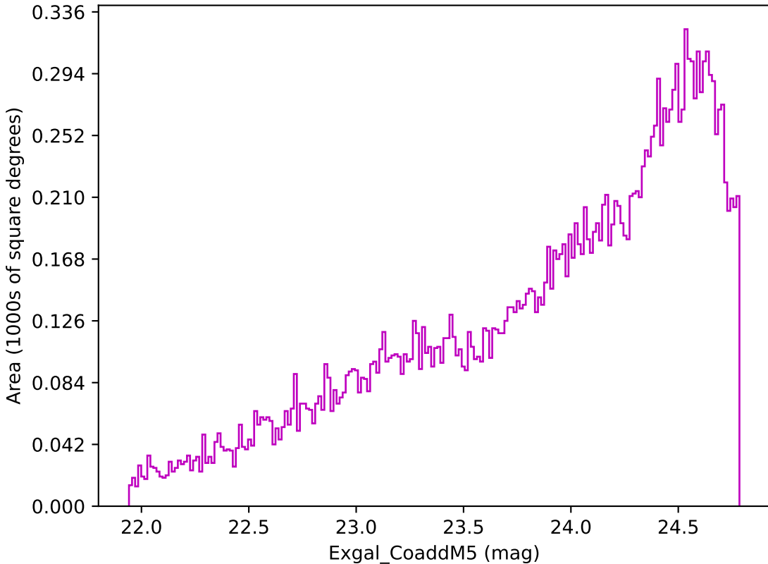
all_long_v3.4_10yrs Yr 3-4 z band: Exgal_CoaddM5
