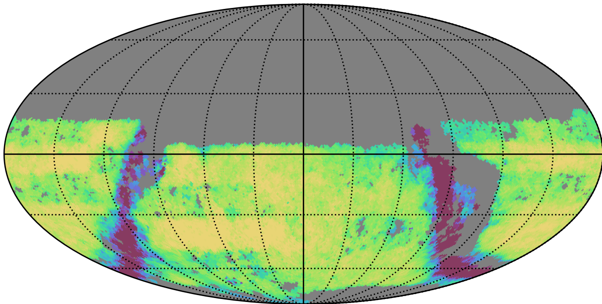
all_long_v3.4_10yrs Yr 3-4 u band: Exgal_CoaddM5
