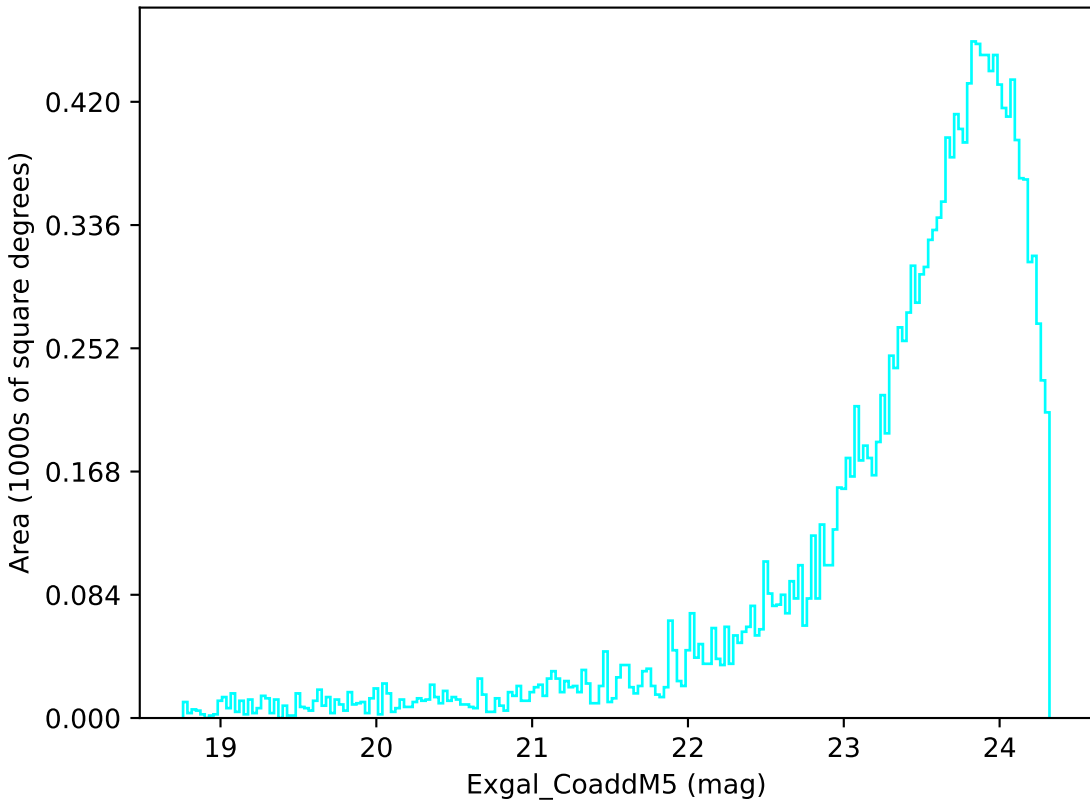
all_long_v3.4_10yrs Yr 3-4 u band: Exgal_CoaddM5
