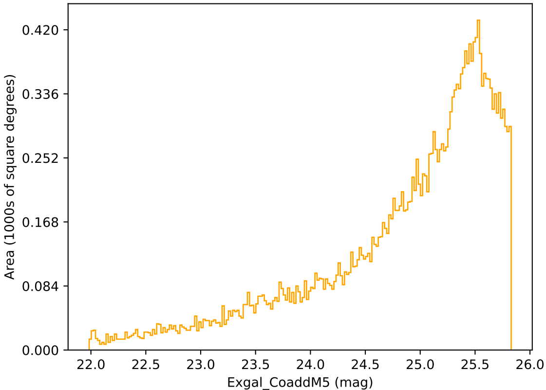
all_long_v3.4_10yrs Yr 3-4 r band: Exgal_CoaddM5
