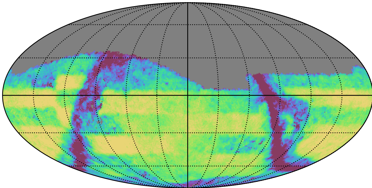
all_long_v3.4_10yrs Yr 3-4 i band: Exgal_CoaddM5
