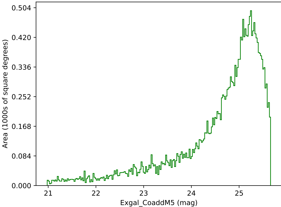
all_long_v3.4_10yrs Yr 3-4 g band: Exgal_CoaddM5
