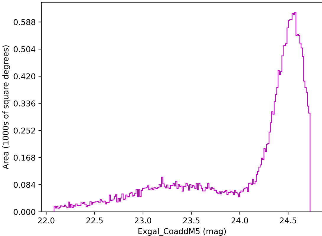
all_long_v3.4_10yrs Yr 1 z band: Exgal_CoaddM5
