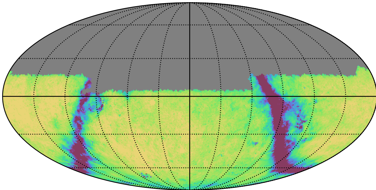
all_long_v3.4_10yrs Yr 1 u band: Exgal_CoaddM5
