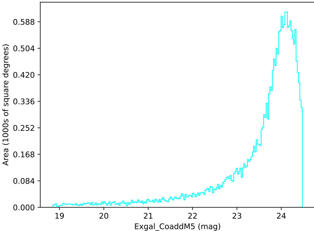
all_long_v3.4_10yrs Yr 1 u band: Exgal_CoaddM5
