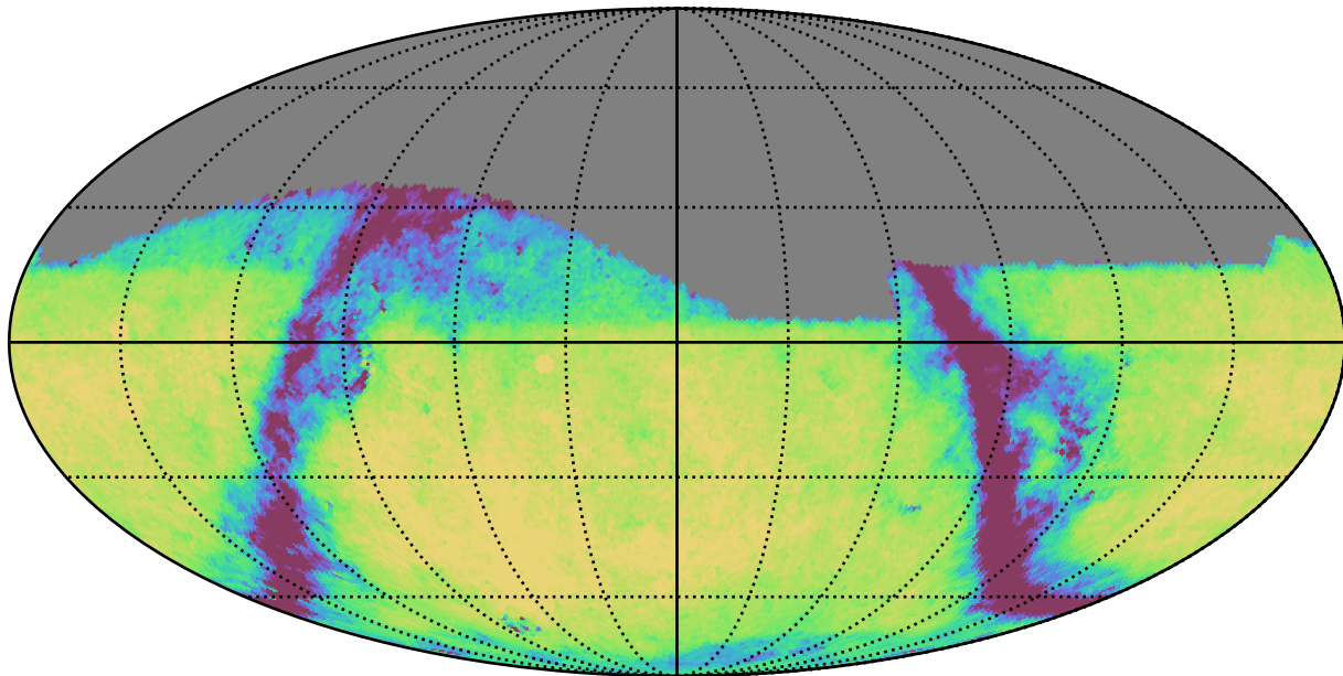
all_long_v3.4_10yrs Yr 1 r band: Exgal_CoaddM5
