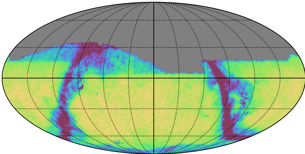
all_long_v3.4_10yrs Yr 1 i band: Exgal_CoaddM5
