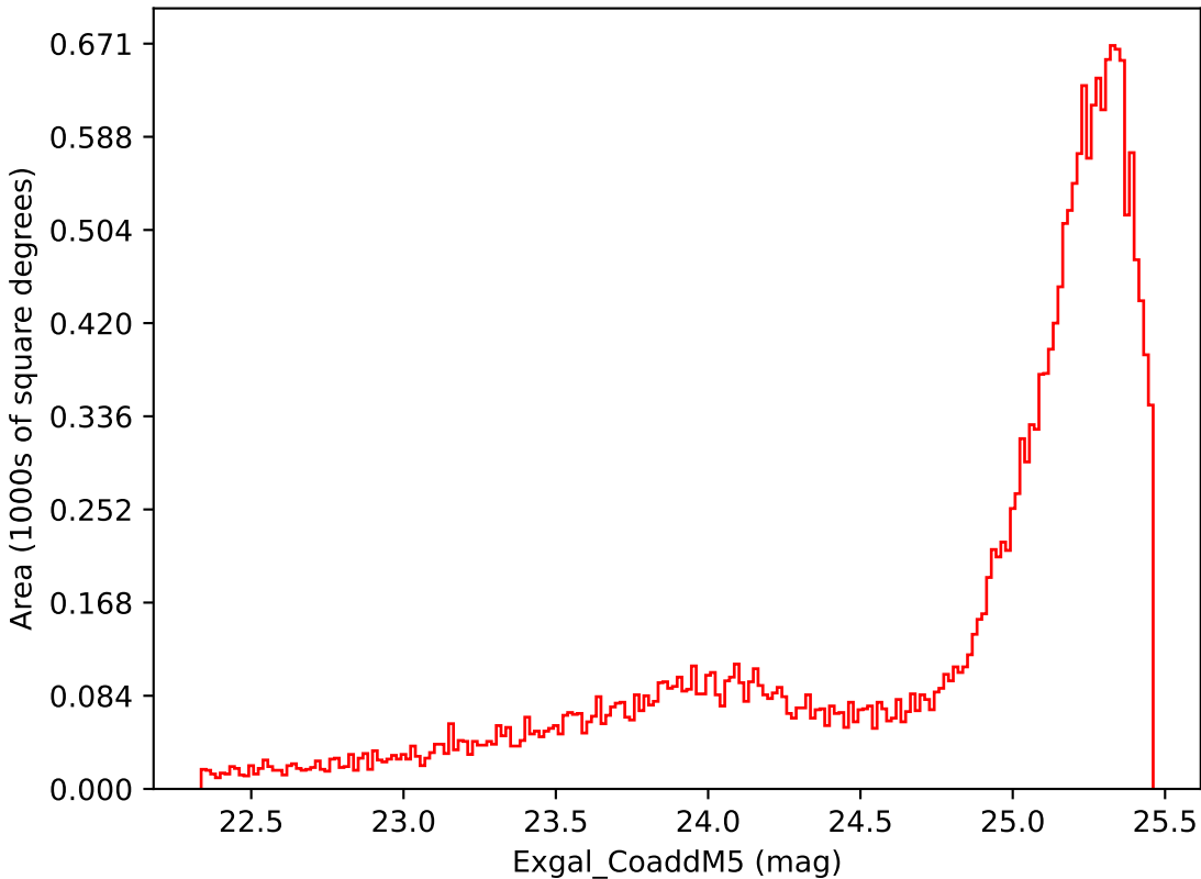
all_long_v3.4_10yrs Yr 1 i band: Exgal_CoaddM5
