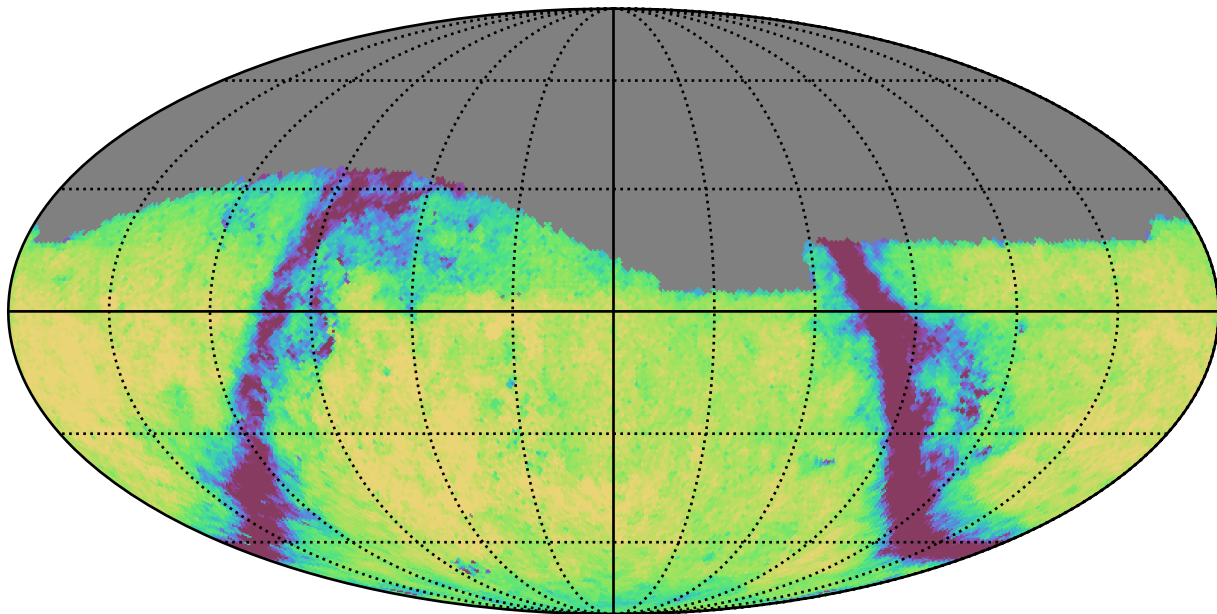
all_long_v3.4_10yrs Yr 1 g band: Exgal_CoaddM5
