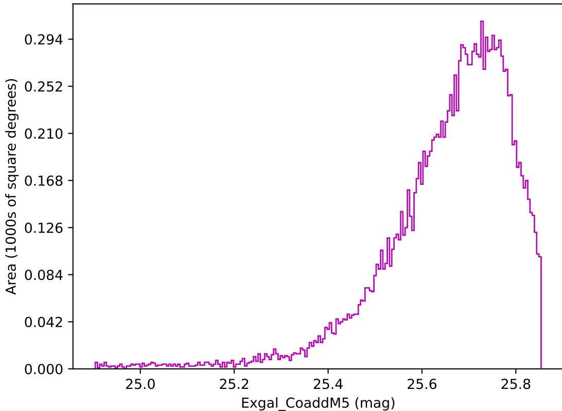
all_long_v3.4_10yrs WFD z band: Exgal_CoaddM5
