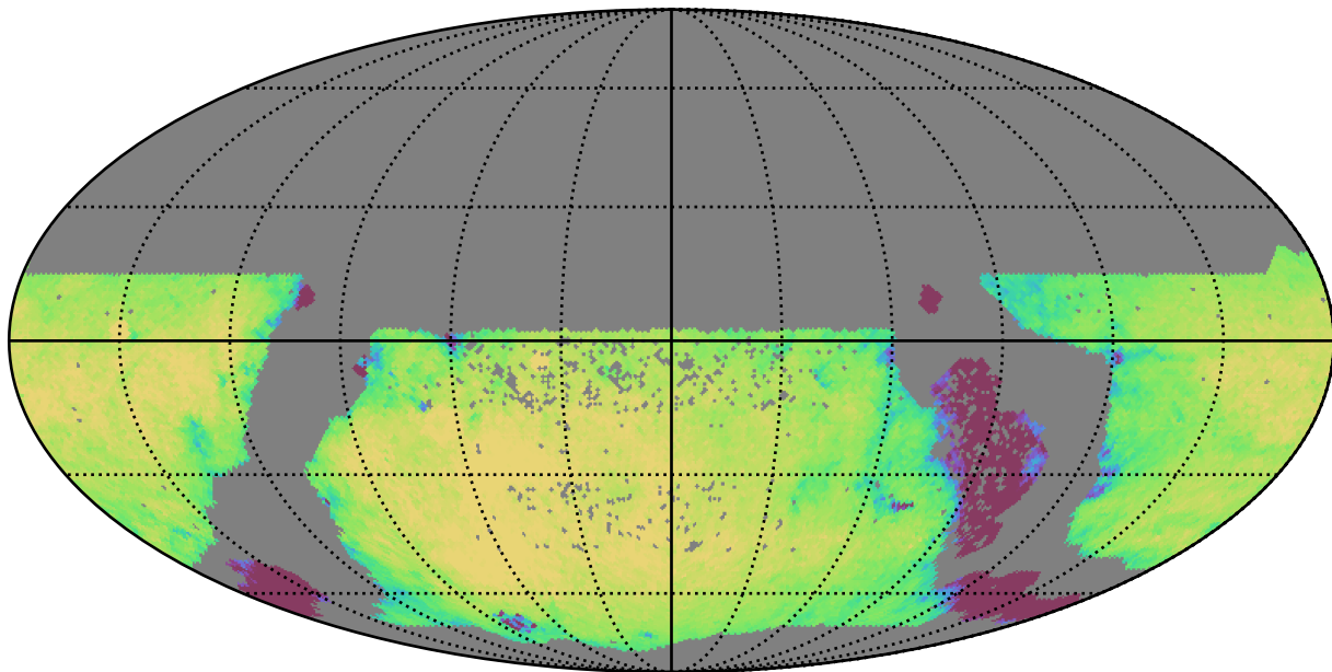
all_long_v3.4_10yrs WFD u band: Exgal_CoaddM5
