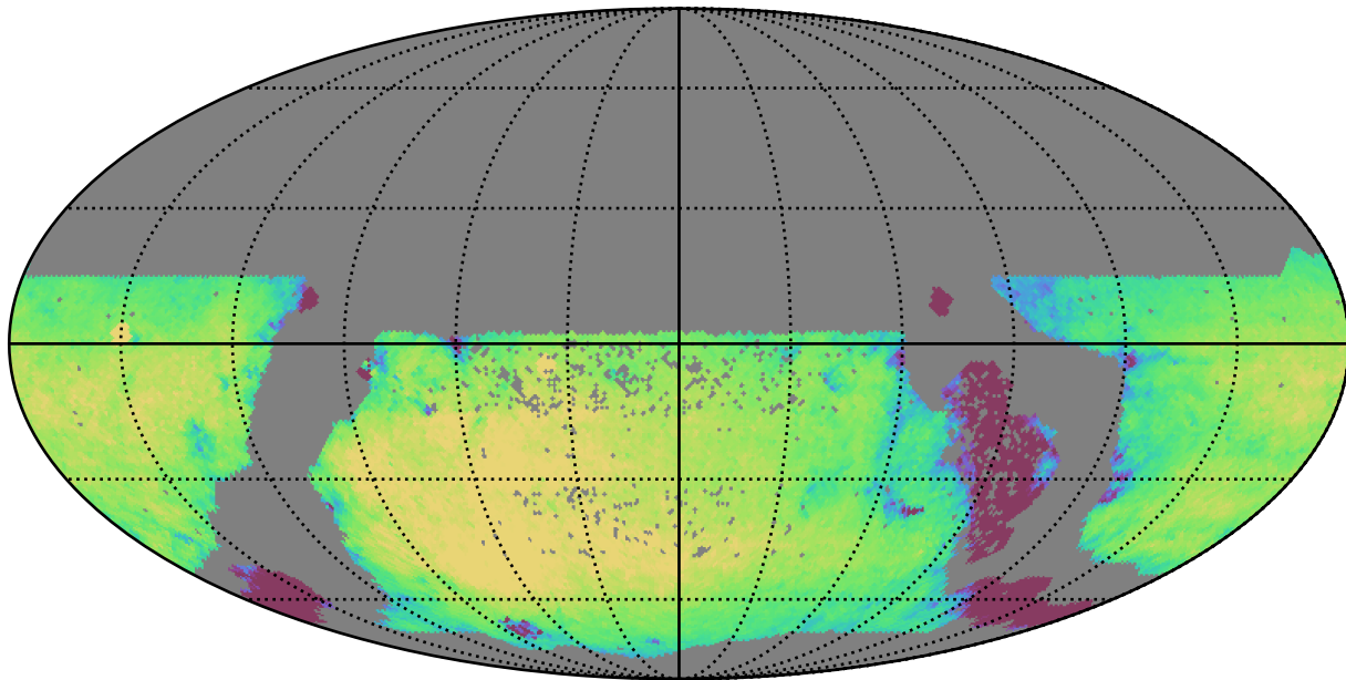
all_long_v3.4_10yrs WFD r band: Exgal_CoaddM5
