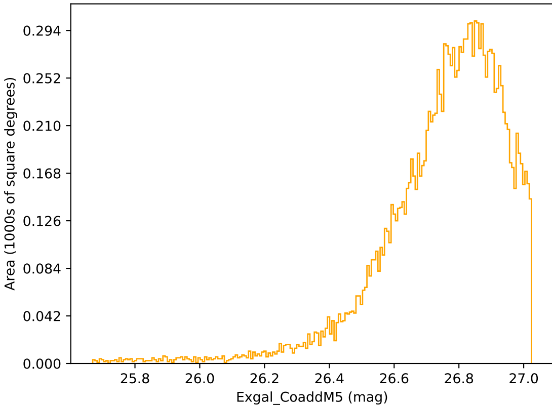
all_long_v3.4_10yrs WFD r band: Exgal_CoaddM5
