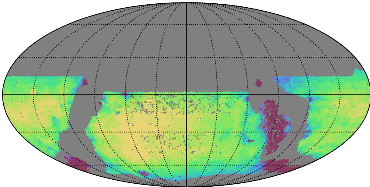
all_long_v3.4_10yrs WFD i band: Exgal_CoaddM5
