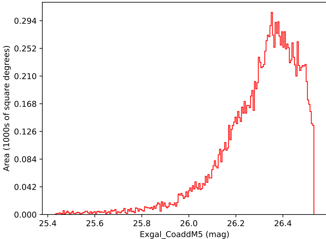
all_long_v3.4_10yrs WFD i band: Exgal_CoaddM5
