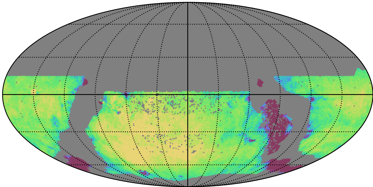
all_long_v3.4_10yrs WFD g band: Exgal_CoaddM5
