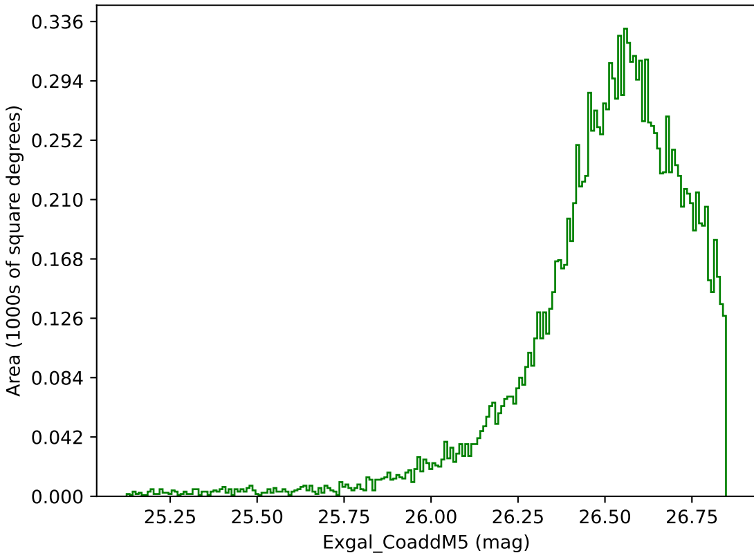
all_long_v3.4_10yrs WFD g band: Exgal_CoaddM5
