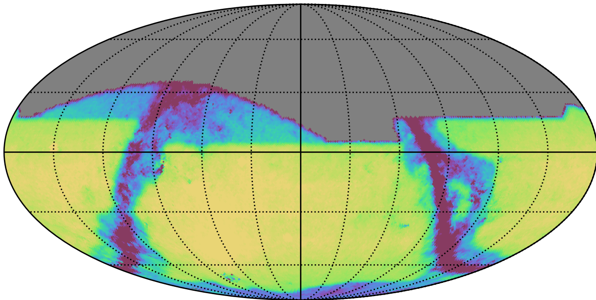
all_long_v3.4_10yrs All sky z band: Exgal_CoaddM5
