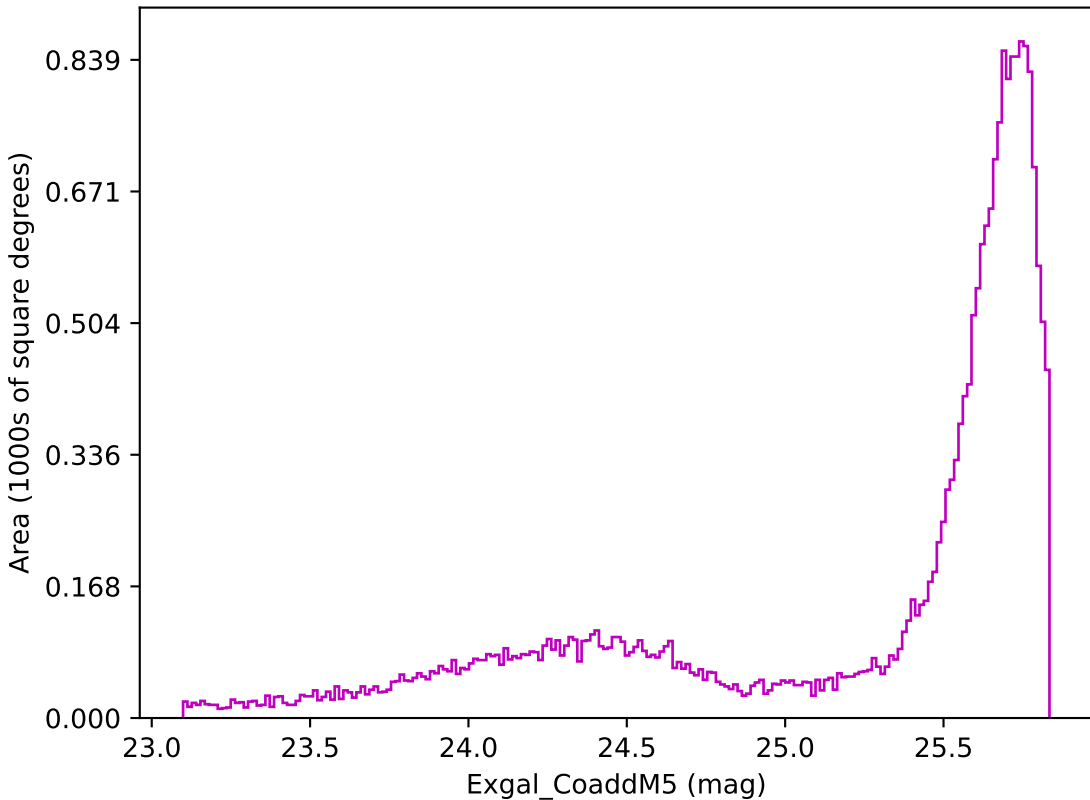
all_long_v3.4_10yrs All sky z band: Exgal_CoaddM5
