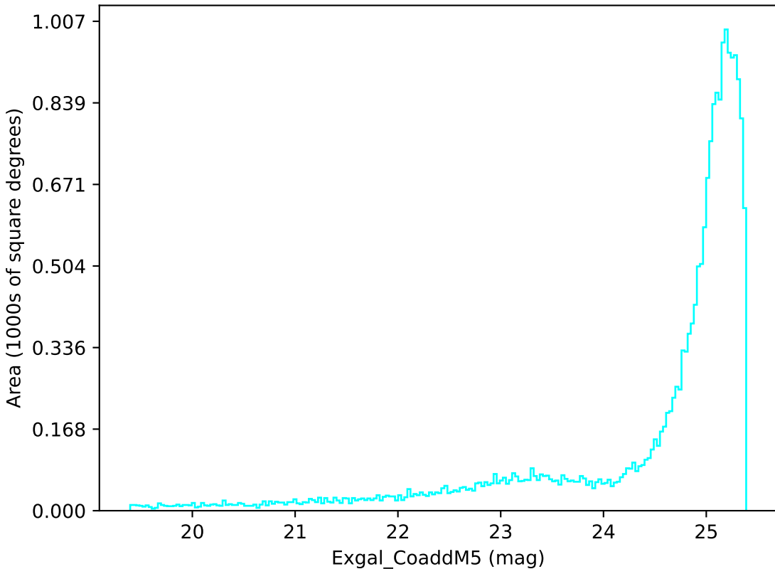
all_long_v3.4_10yrs All sky u band: Exgal_CoaddM5
