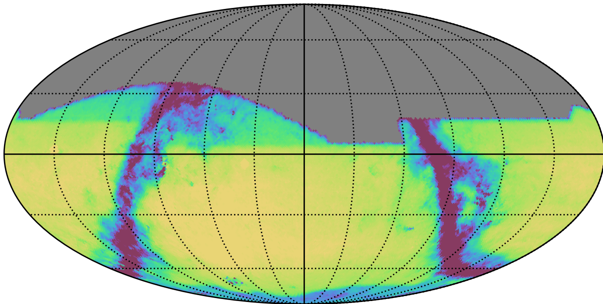
all_long_v3.4_10yrs All sky r band: Exgal_CoaddM5
