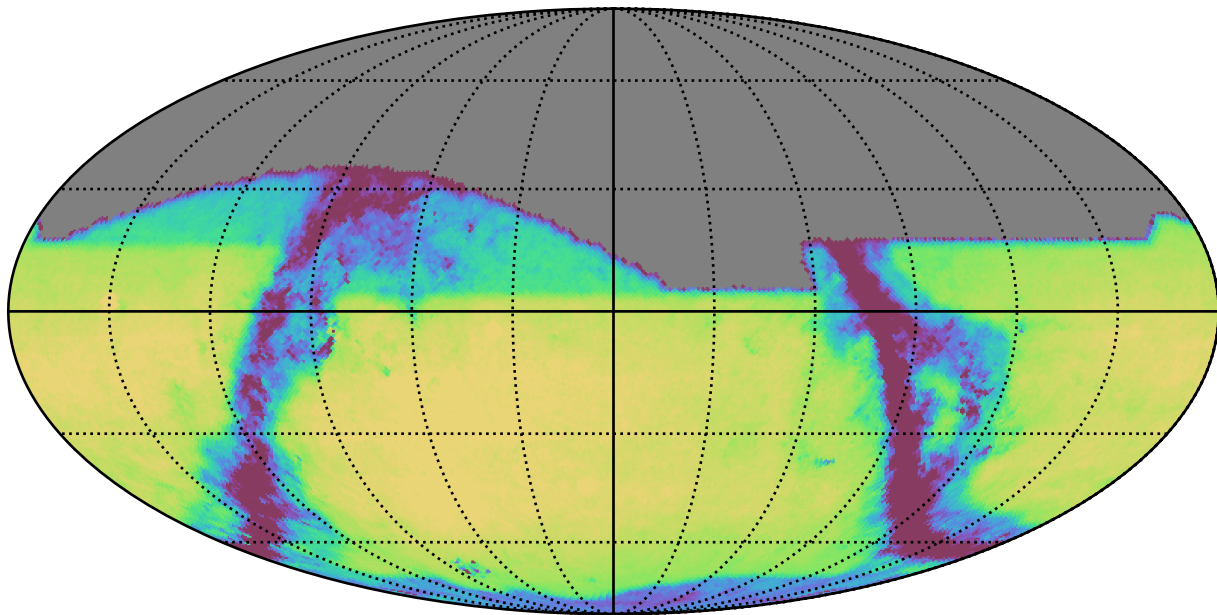
all_long_v3.4_10yrs All sky i band: Exgal_CoaddM5
