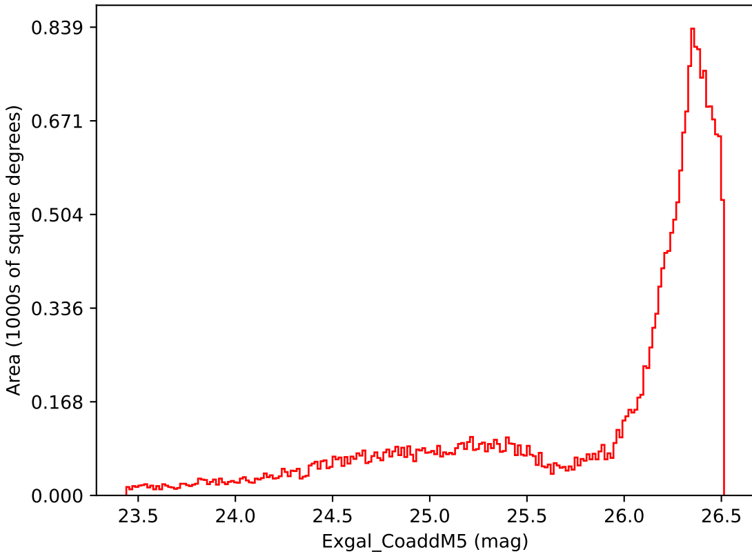
all_long_v3.4_10yrs All sky i band: Exgal_CoaddM5
