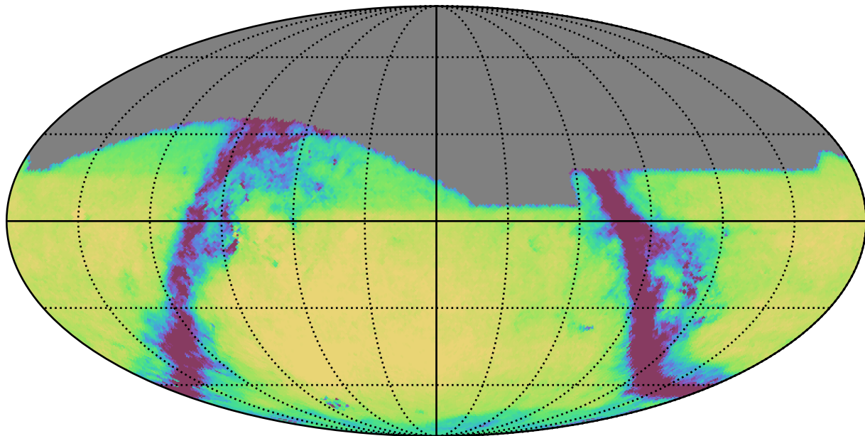
all_long_v3.4_10yrs All sky g band: Exgal_CoaddM5
