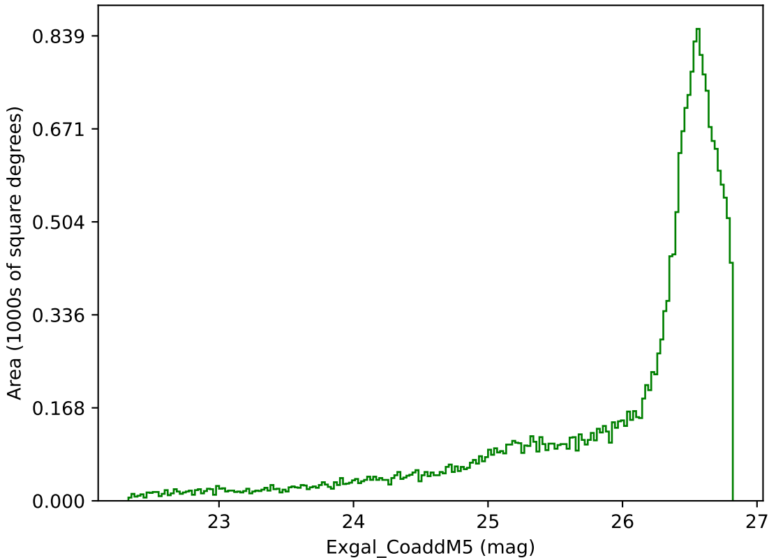
all_long_v3.4_10yrs All sky g band: Exgal_CoaddM5
