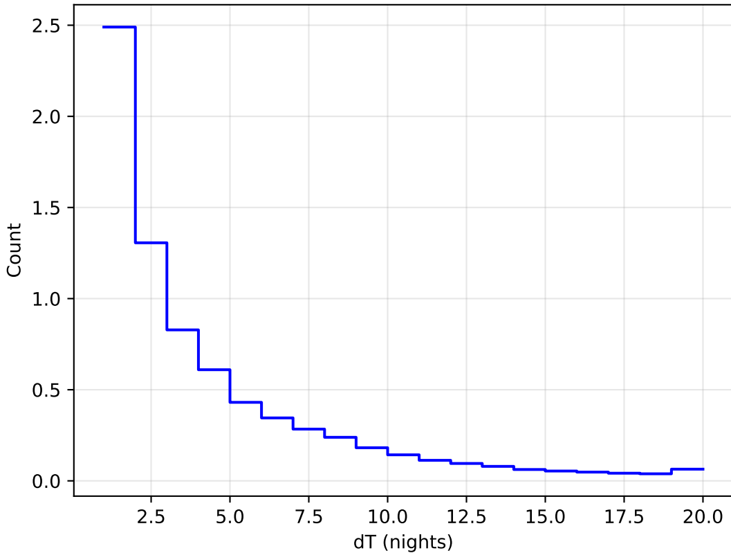
all_long_v3.4_10yrs WFD all bands: DeltaNight Histogram 1e6
