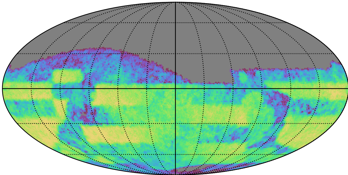
all_long_v3.4_10yrs Yr 3-4 z band: CoaddM5
