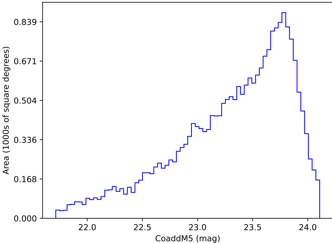
all_long_v3.4_10yrs Yr 3-4 y band: CoaddM5
