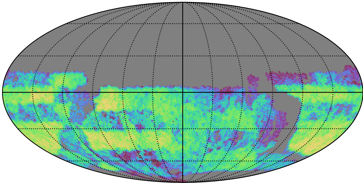
all_long_v3.4_10yrs Yr 3-4 u band: CoaddM5
