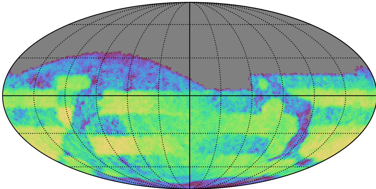
all_long_v3.4_10yrs Yr 3-4 r band: CoaddM5
