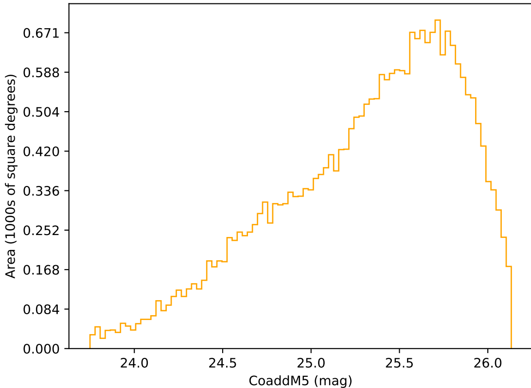
all_long_v3.4_10yrs Yr 3-4 r band: CoaddM5
