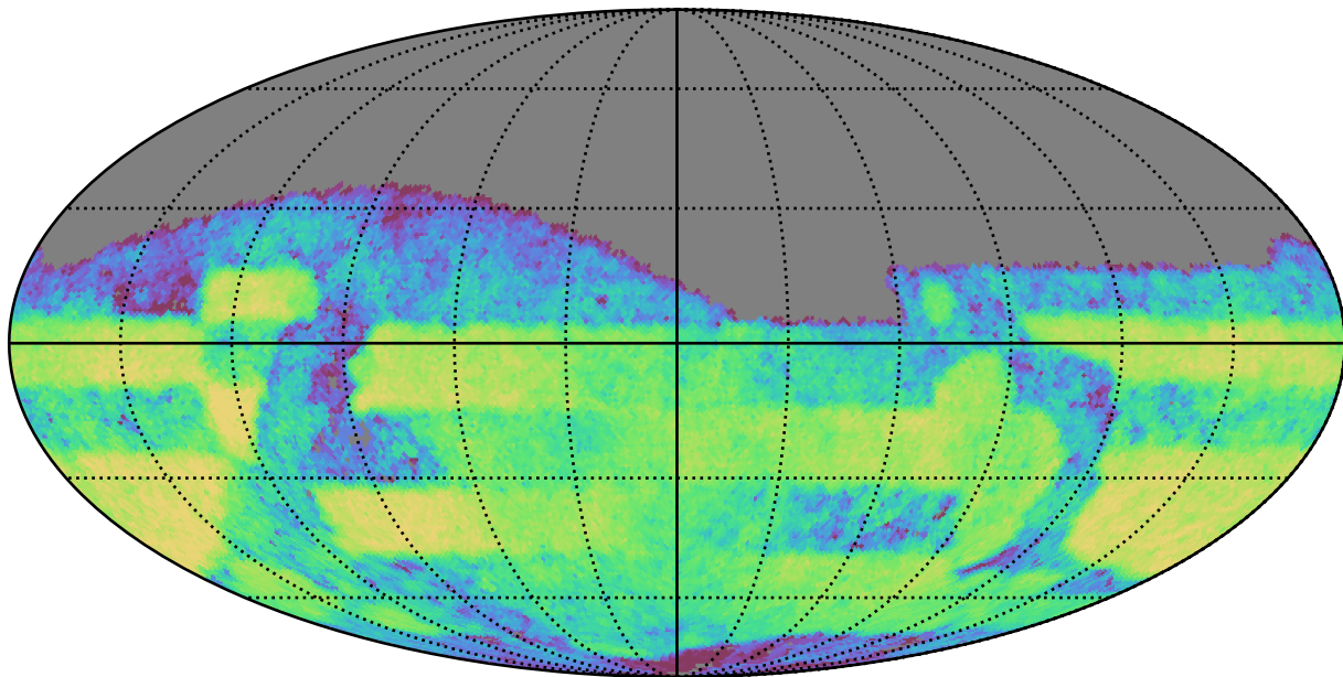
all_long_v3.4_10yrs Yr 3-4 i band: CoaddM5
