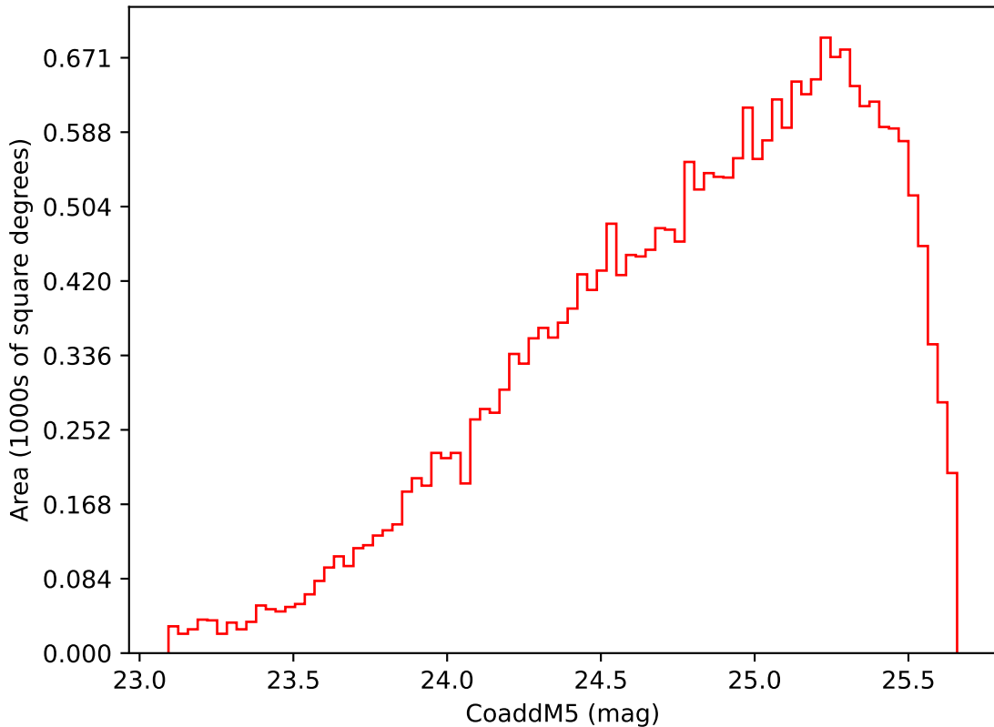
all_long_v3.4_10yrs Yr 3-4 i band: CoaddM5
