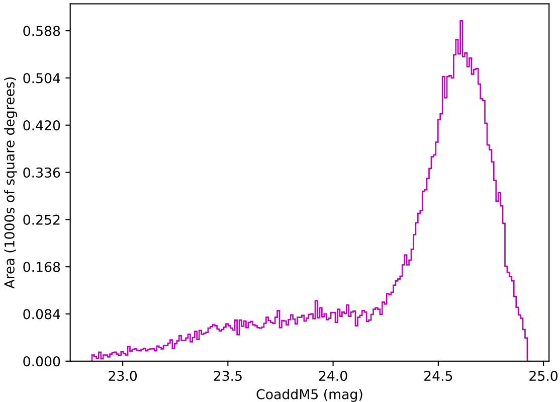
all_long_v3.4_10yrs Yr 1 z band: CoaddM5
