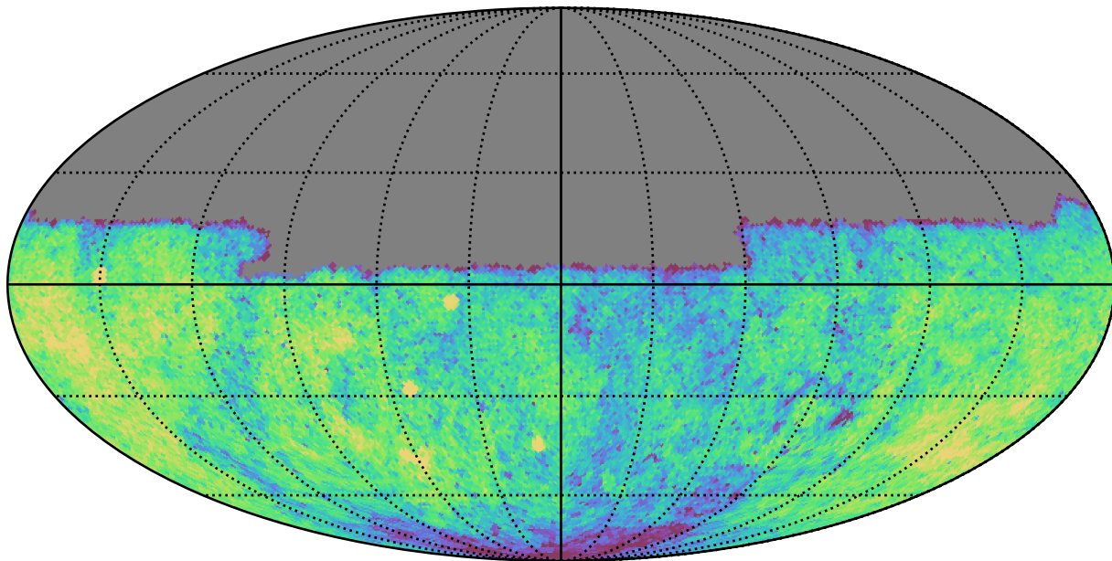
all_long_v3.4_10yrs Yr 1 u band: CoaddM5
