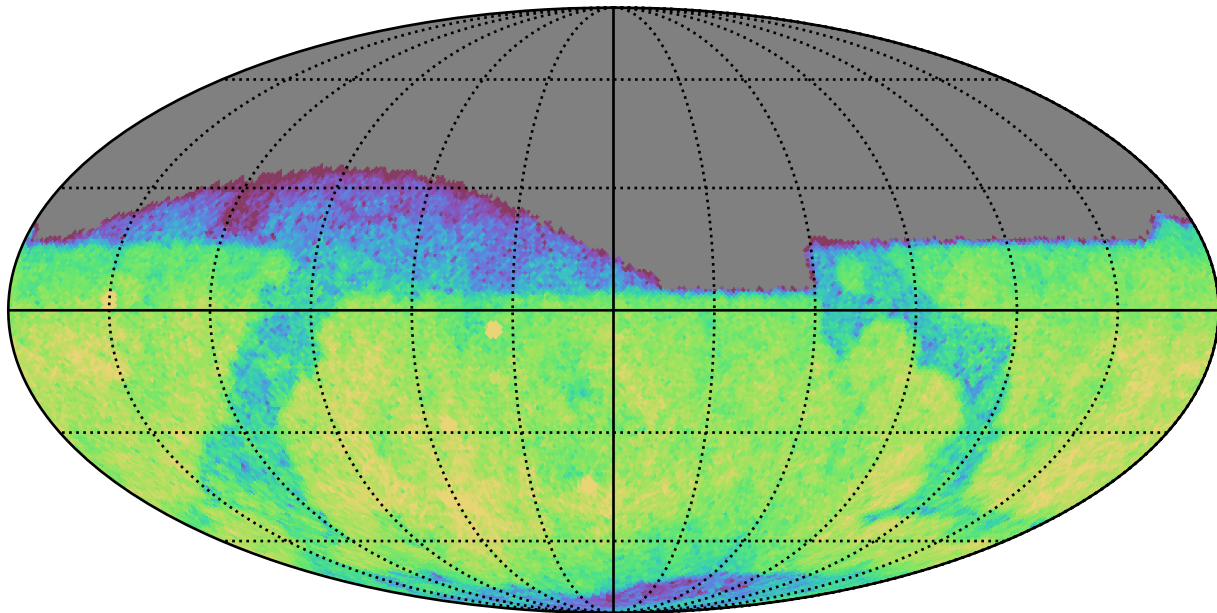
all_long_v3.4_10yrs Yr 1 r band: CoaddM5
