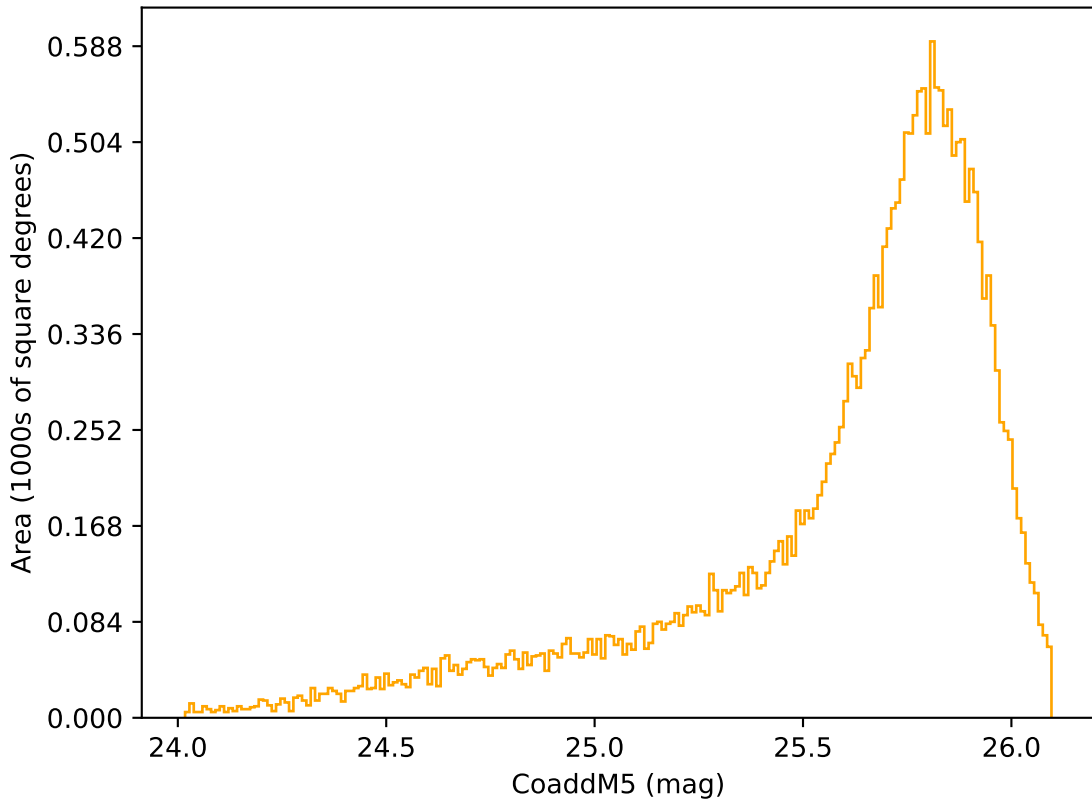
all_long_v3.4_10yrs Yr 1 r band: CoaddM5
