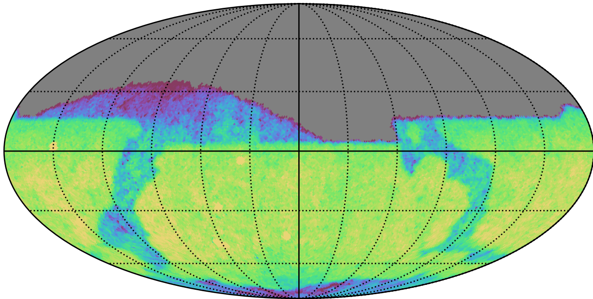
all_long_v3.4_10yrs Yr 1 i band: CoaddM5
