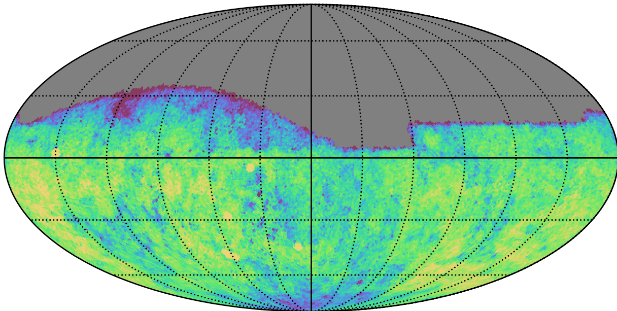
all_long_v3.4_10yrs Yr 1 g band: CoaddM5
