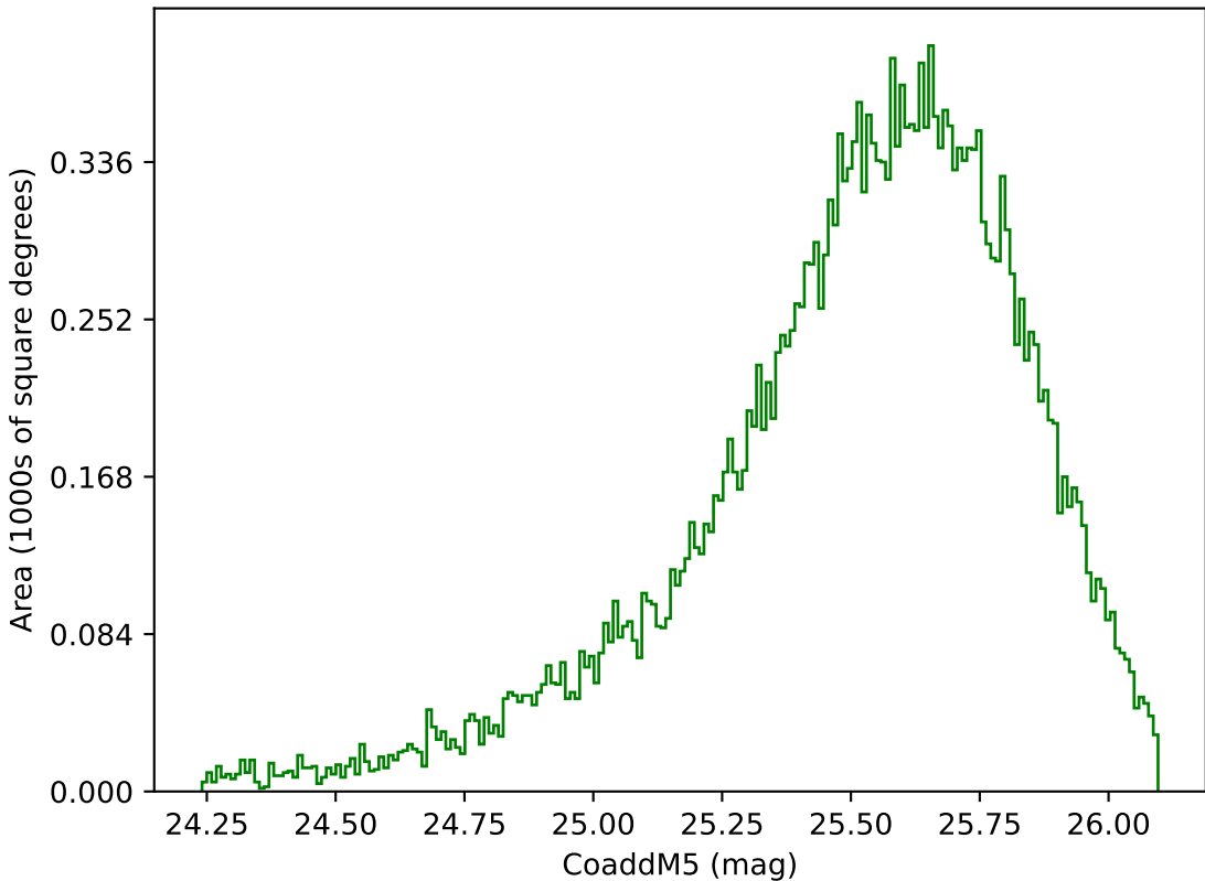
all_long_v3.4_10yrs Yr 1 g band: CoaddM5
