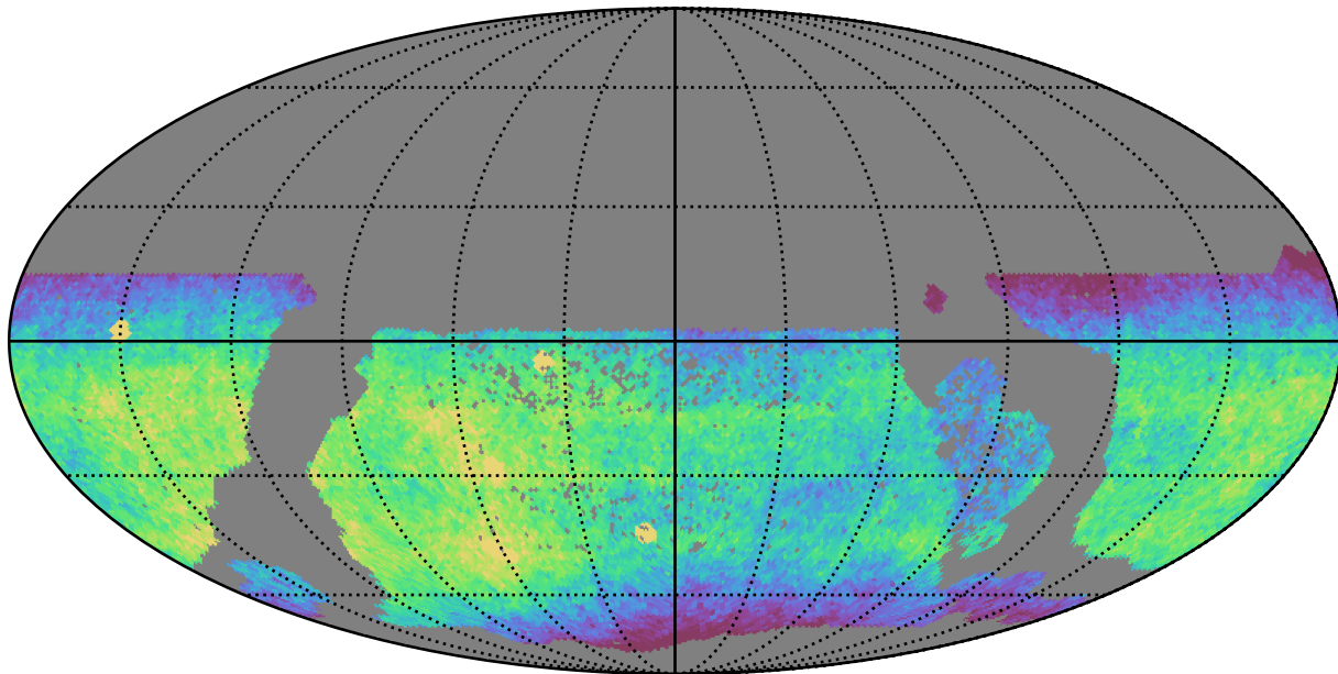
all_long_v3.4_10yrs WFD z band: CoaddM5
