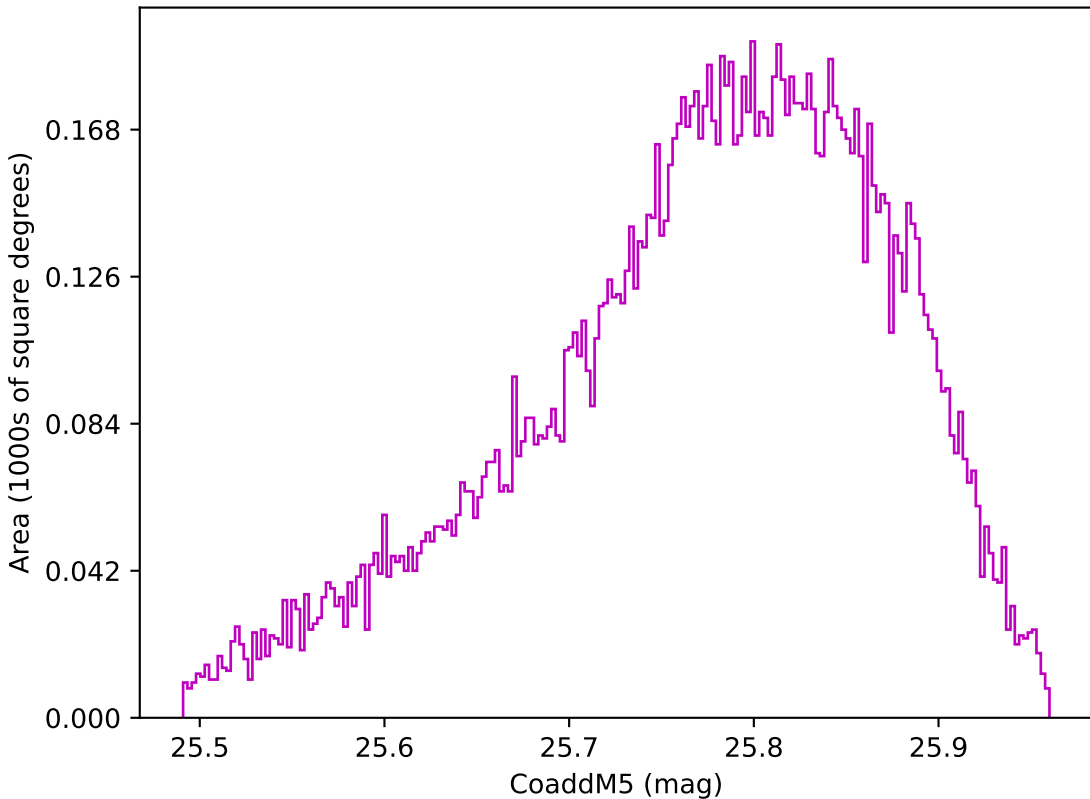
all_long_v3.4_10yrs WFD z band: CoaddM5
